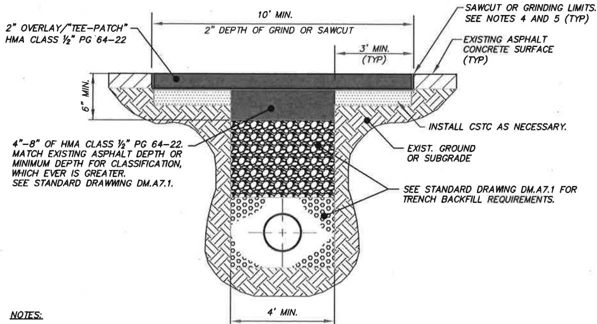
SECTION
